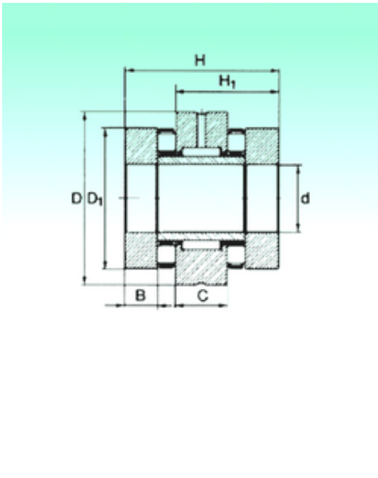
ZARN 3062 TN Bearing 2D drawings and 3D CAD models
